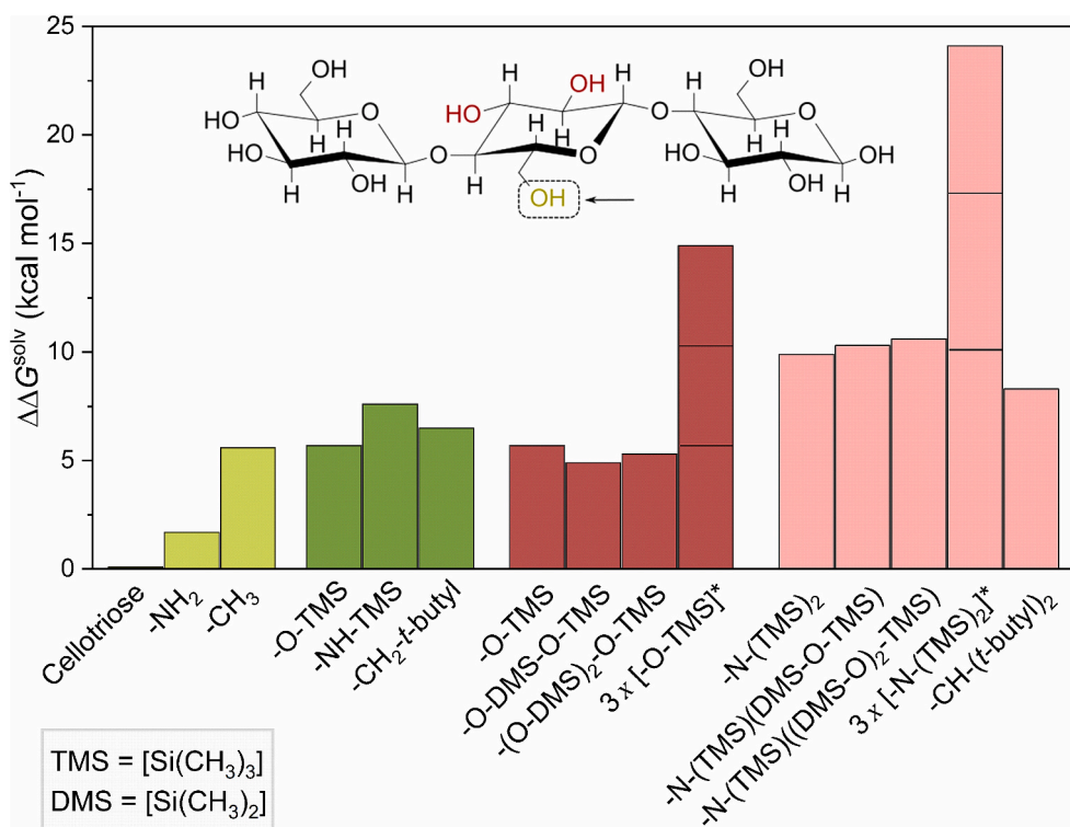
Fig. 7. Changes in free energy of solvation as the OH group on C 6 (circled) in cellulose is substituted. A more positive value represents greater hydrophobicity. Various t -butyl substituents are used as model compounds for inert hydrophobic groups of comparable steric hindrance. Asterisk (*) denote that all three (C 2 , C 3 , C 6 ) OH groups are substituted, showing that the effect is additive.
